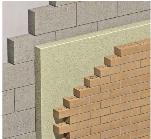
Figure 02: insulating masonry walls
